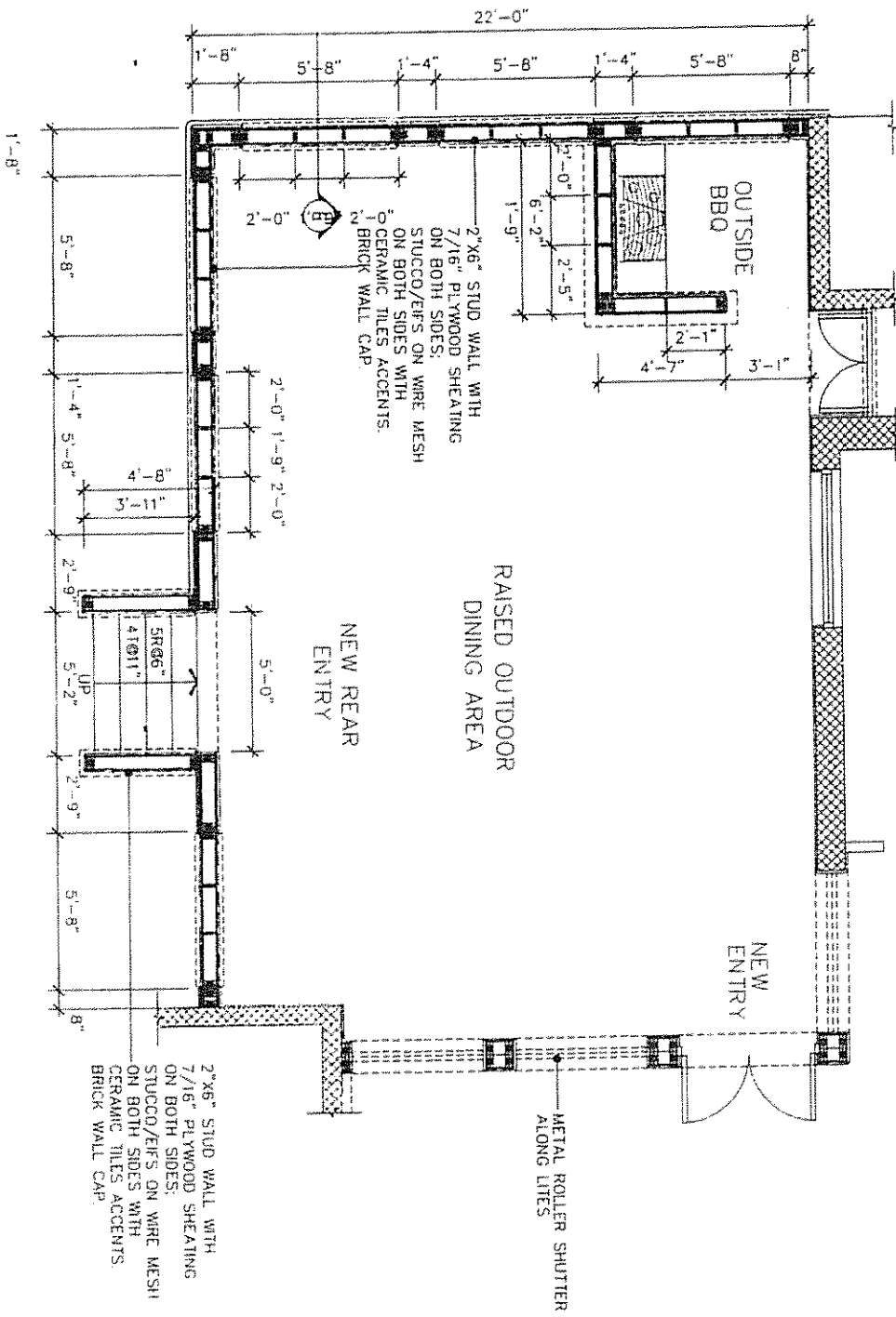
PLAN DETAIL 2 SCALE 1/8"=1'-0"
